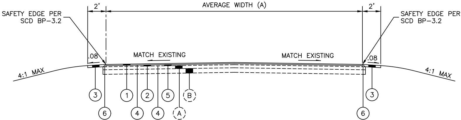
TYPICAL SECTION CR 165 NOT TO SCALE
