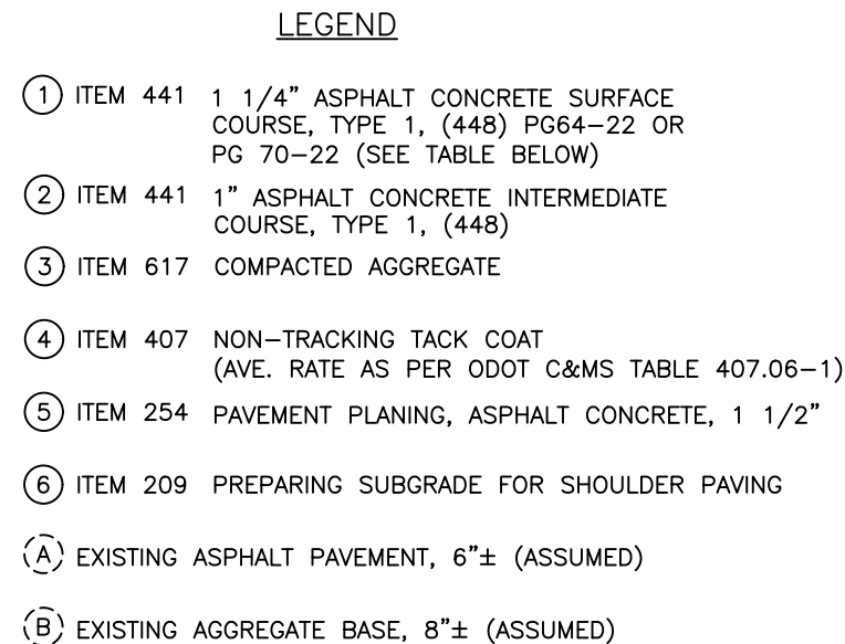
NOTE: TYPICAL SECTION EXCLUDES ADDITIONAL WIDTH OF TURN LANES.
